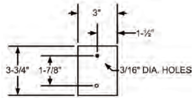
Mounting Plate Dimensions and Hole Locations
