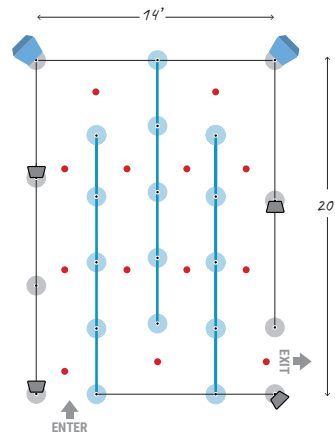
4 Lane Queue 14' x 20' Footprint
