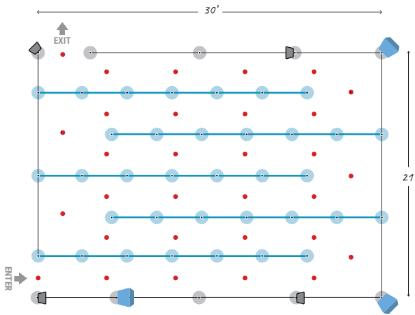
7 Lane Queue 30' x 21' Footprint
