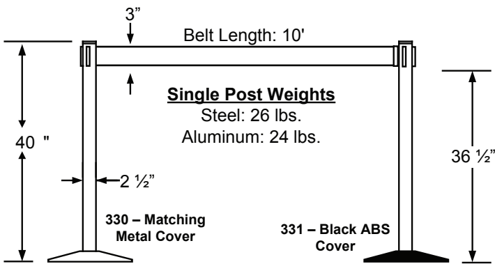
Specs for 10' Single Line RETRACTA-BELT® with 3" Belt (other post models available)
