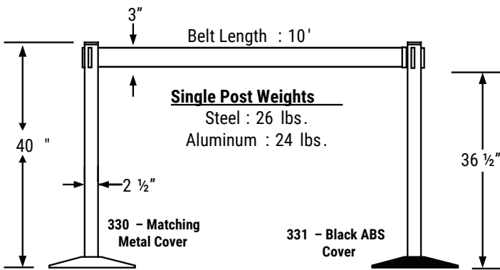
Specs for 10' Single Line RETRACTA-BELT® with 3" Belt (other post models available)
